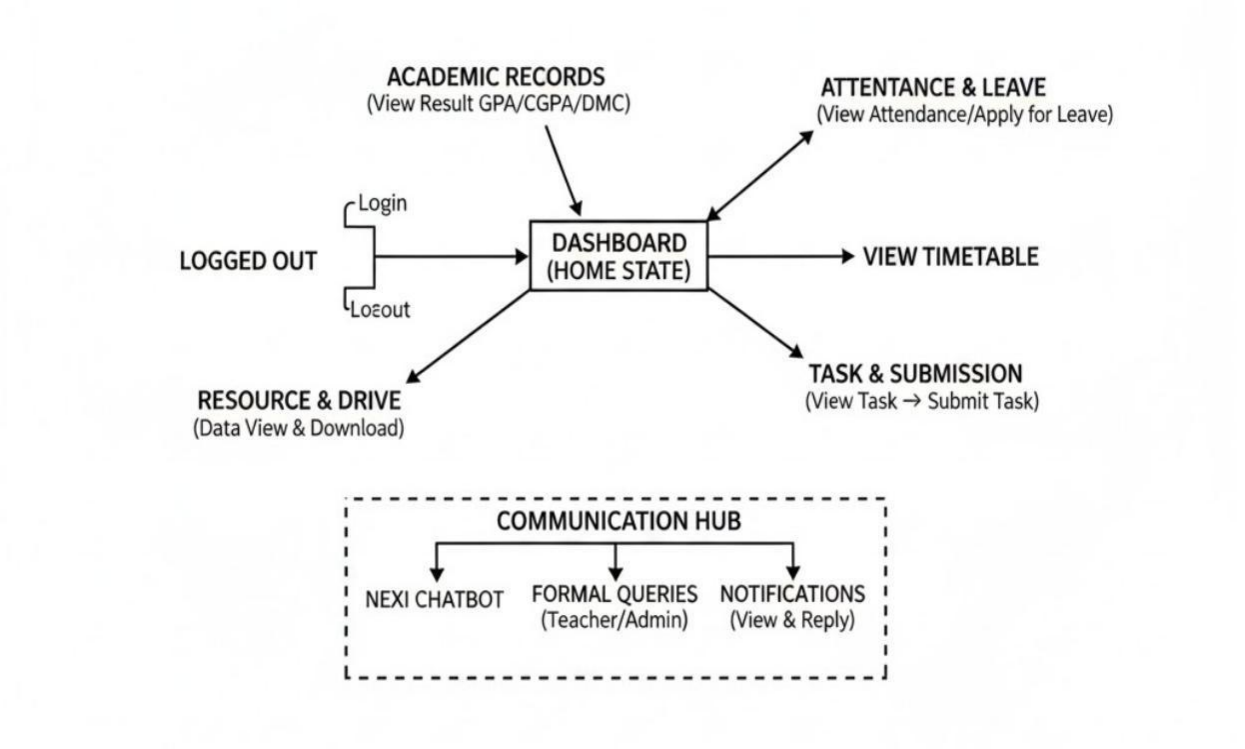
Figure 5.7: Student State Diagram
