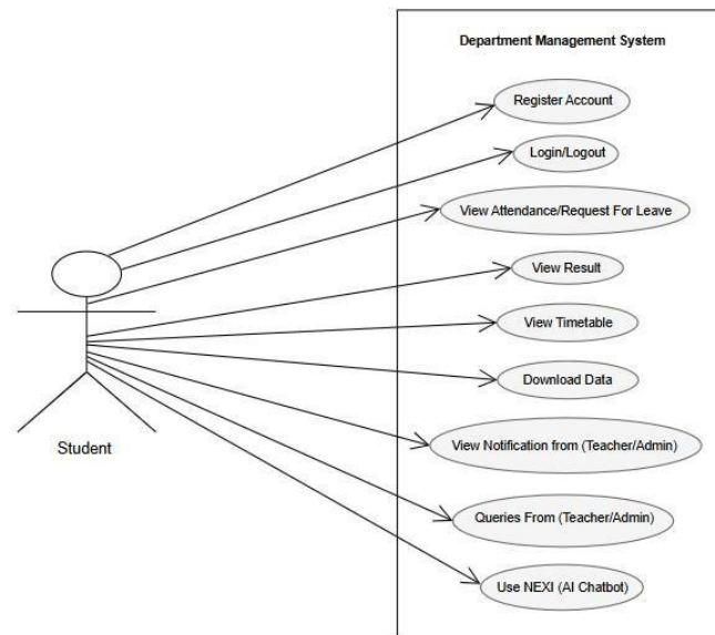
Figure 4.1: Student Use Case Diagram
