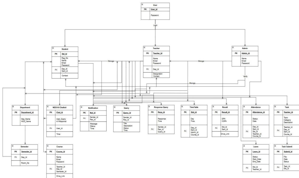
Figure 5.1: Database Diagram
