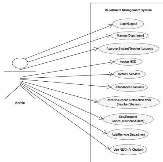
Figure 4.3: Admin Use Case Diagram
