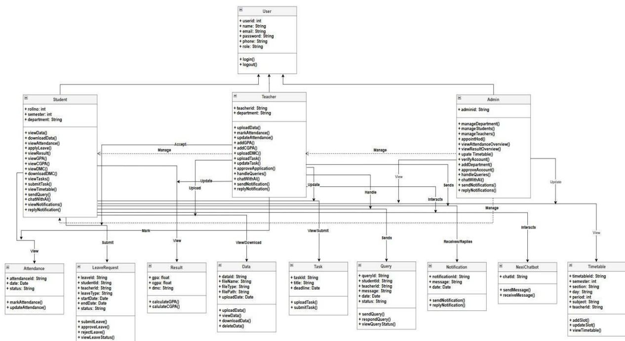
Figure 5.3: Class Diagram
